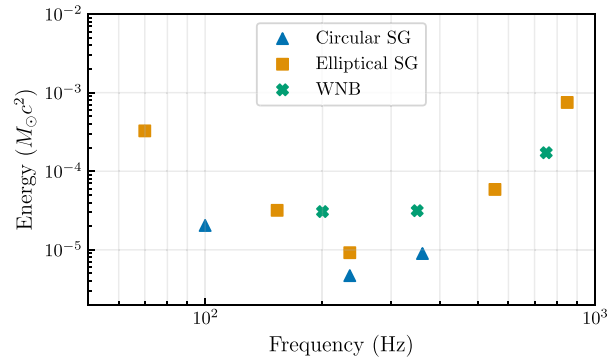
Fig. 6. The GW emitted energy in units of solar masses ( M_{\odot}c^2 ) that correspond to a 50% detection efficiency with cWB at an iFAR of \geq 1 year, for a source located at 10 kpc. The circular SG waveforms are indicated by triangles, the elliptical SG waveforms by squares, and the WNB waveforms by crosses.
